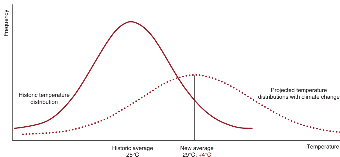
FIGURE 1.1. ILLUSTRATION OF THE EVOLUTION OF A TEMPERATURE DISTRIBUTION WITH A +4°C CHANGE IN AVERAGE TEMPERATURE
